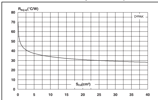
Figure 11. Thermal resistance junction to ambient versus copper surface under tab (epoxy printed board FR4, Cu = 35 \mu m - D 2 PAK)
